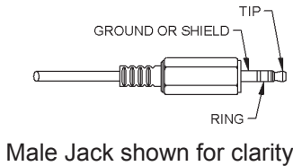
Fig 4: C35L Communications Jack
