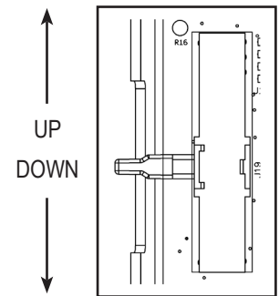
Fig 12: R16 Slide Potentiometer (for making program adjustments)
