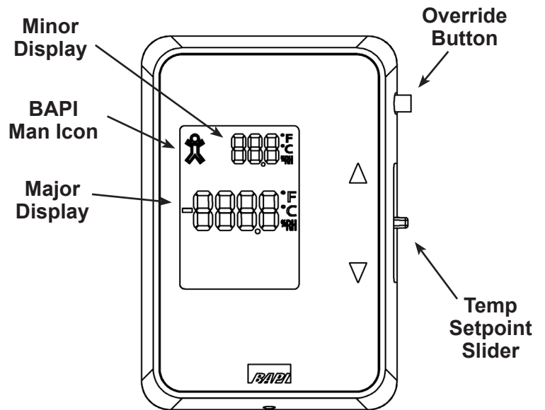
Fig 9: BAPI-Stat “Quantum” Humidity Unit Indicators (Shown with all optional indicators)
