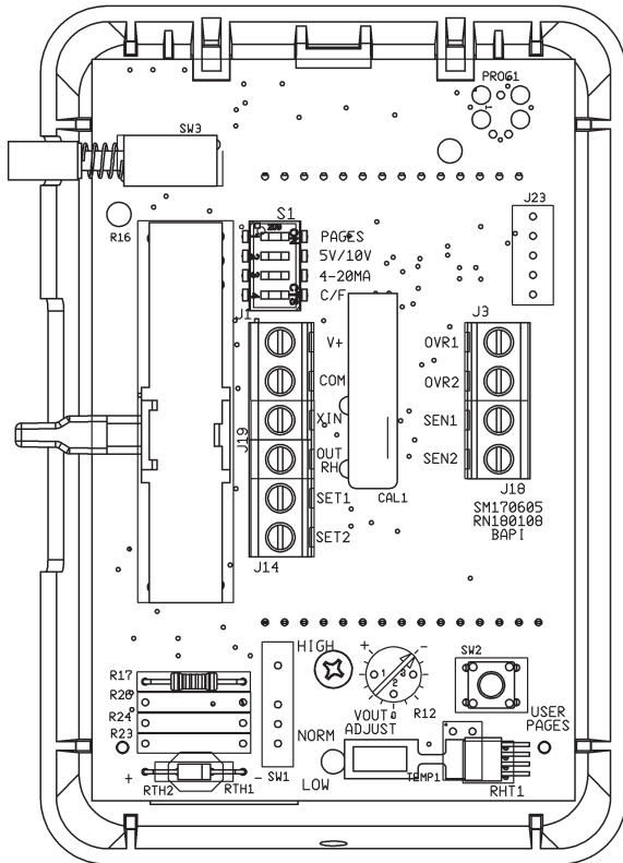
Fig 3: Circuit Board
